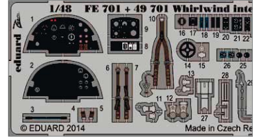
FE701 Whirlwind interior S.A. 1/48 Trumpeter (1 часть)
