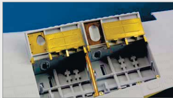
23021 Typhoon Mk.Ib wing armament 1/24 Airfix (1 часть)
